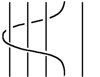
Figure 5: The braid \eta_{4,6}
