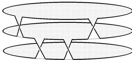
Figure 3: Seifert surface of a braid
