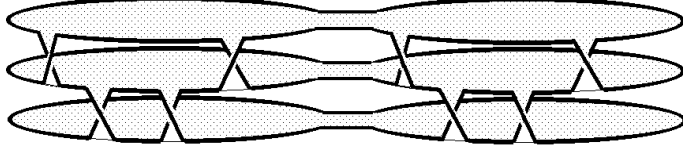
Figure 4: Signature is a quasimorphism
