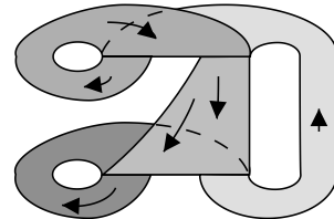
Figure 4. The Ghrist template
