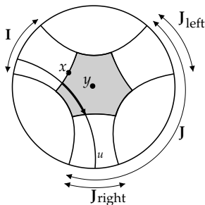
Figure 7. Universal cover of \Sigma_\rho
