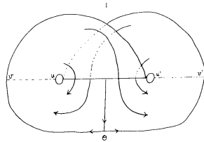
Figure 3. The Lorenz template
