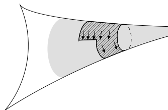
Figure 10. Cusp neighborhood
