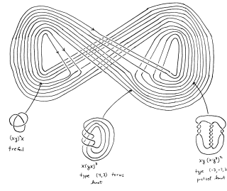
Figure 2. Some periodic orbits [17]
