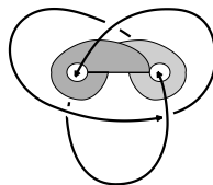
Figure 11. Trefoil wearing modular glasses
